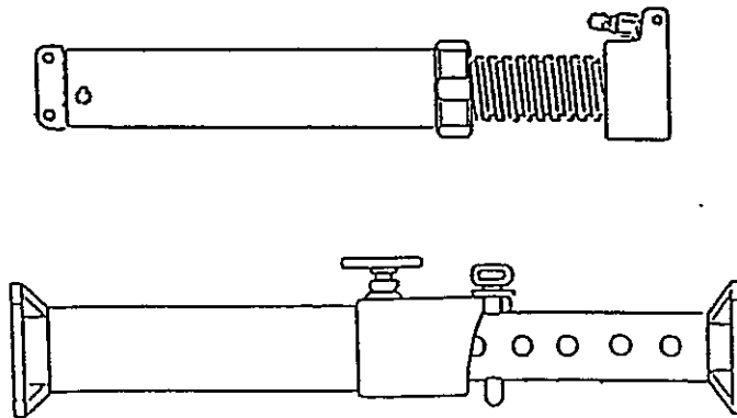
Figure 2. Pneumatic/Hydraulic Shoring
