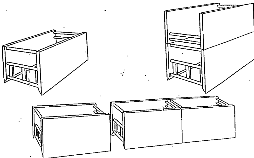
Figure 4. Trench Shields
