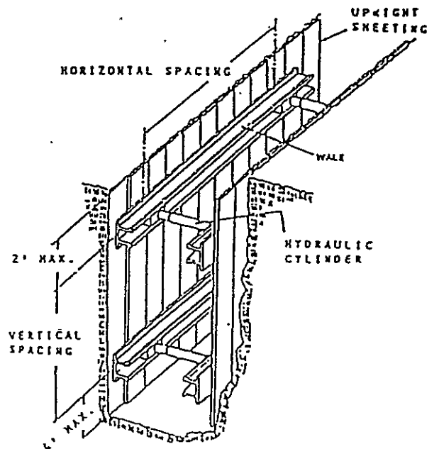
Figure No. 4 Aluminum hydraulic shoring - Water System (typical)
