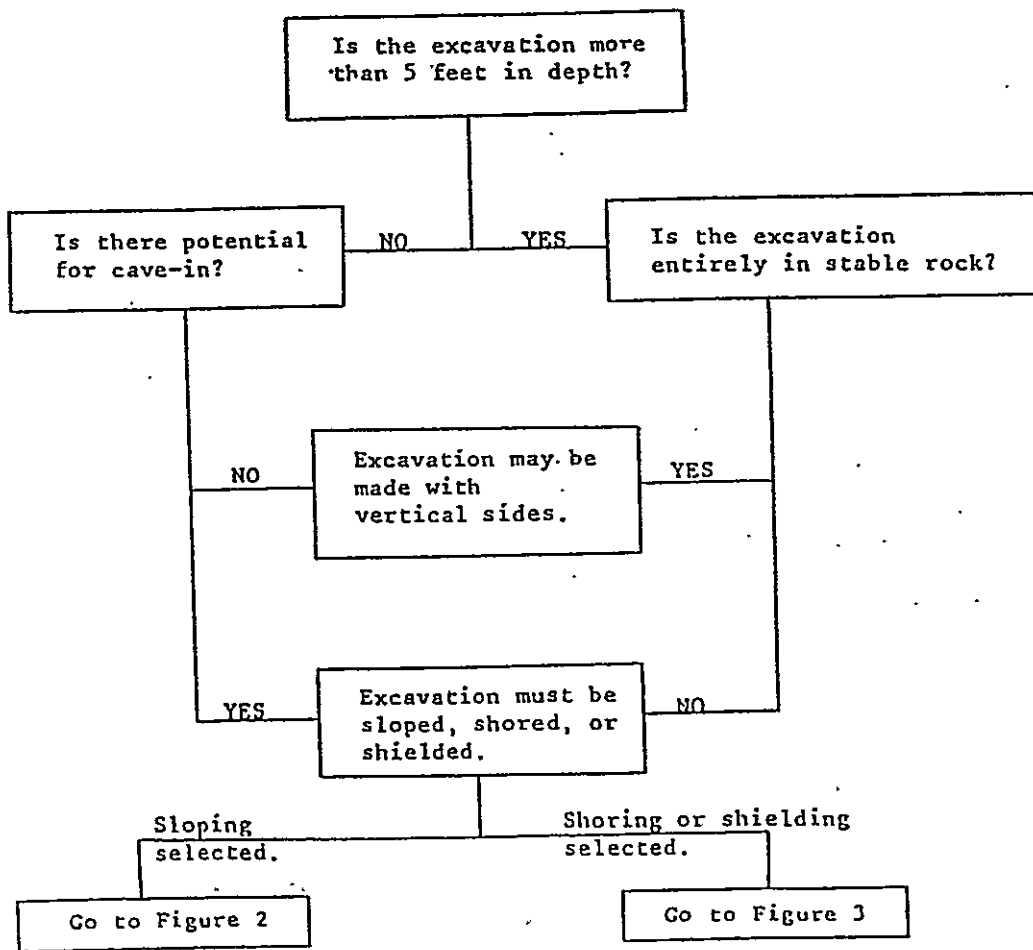
Figure 1. Preliminary Decisions
